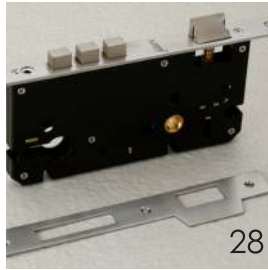
Lock Body & Cylinder
